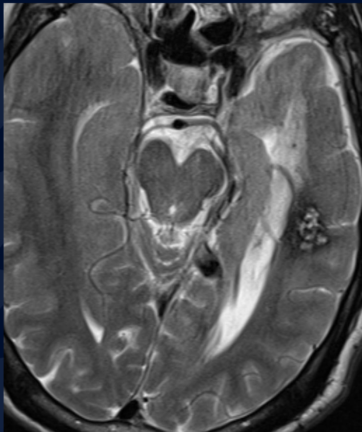
T2 Axial
