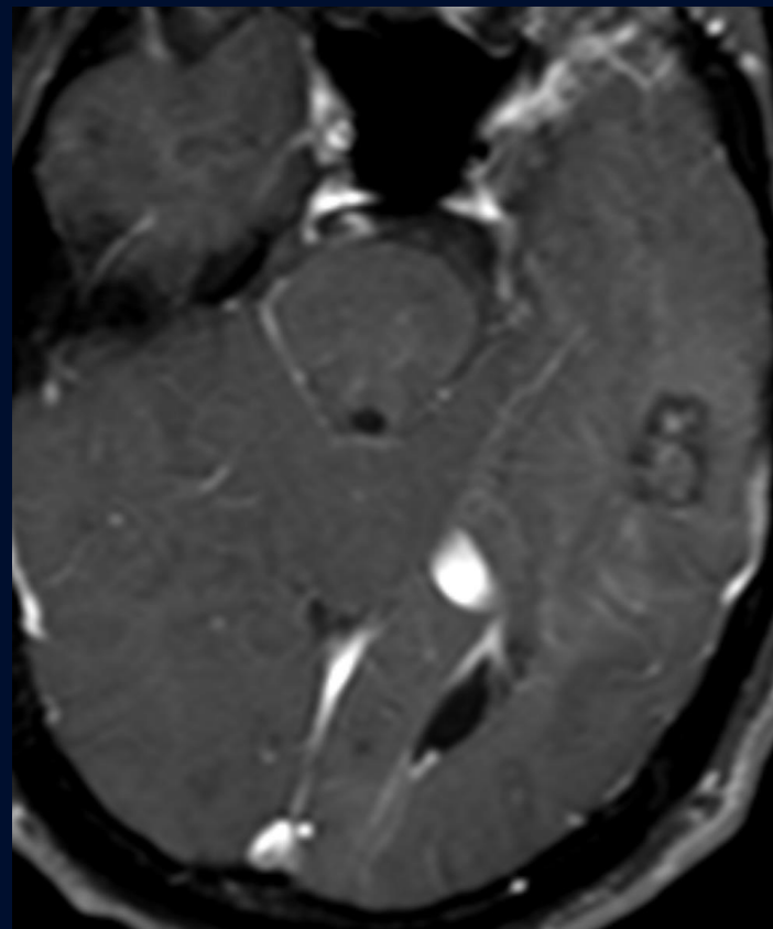
Gd-T1 Axial
