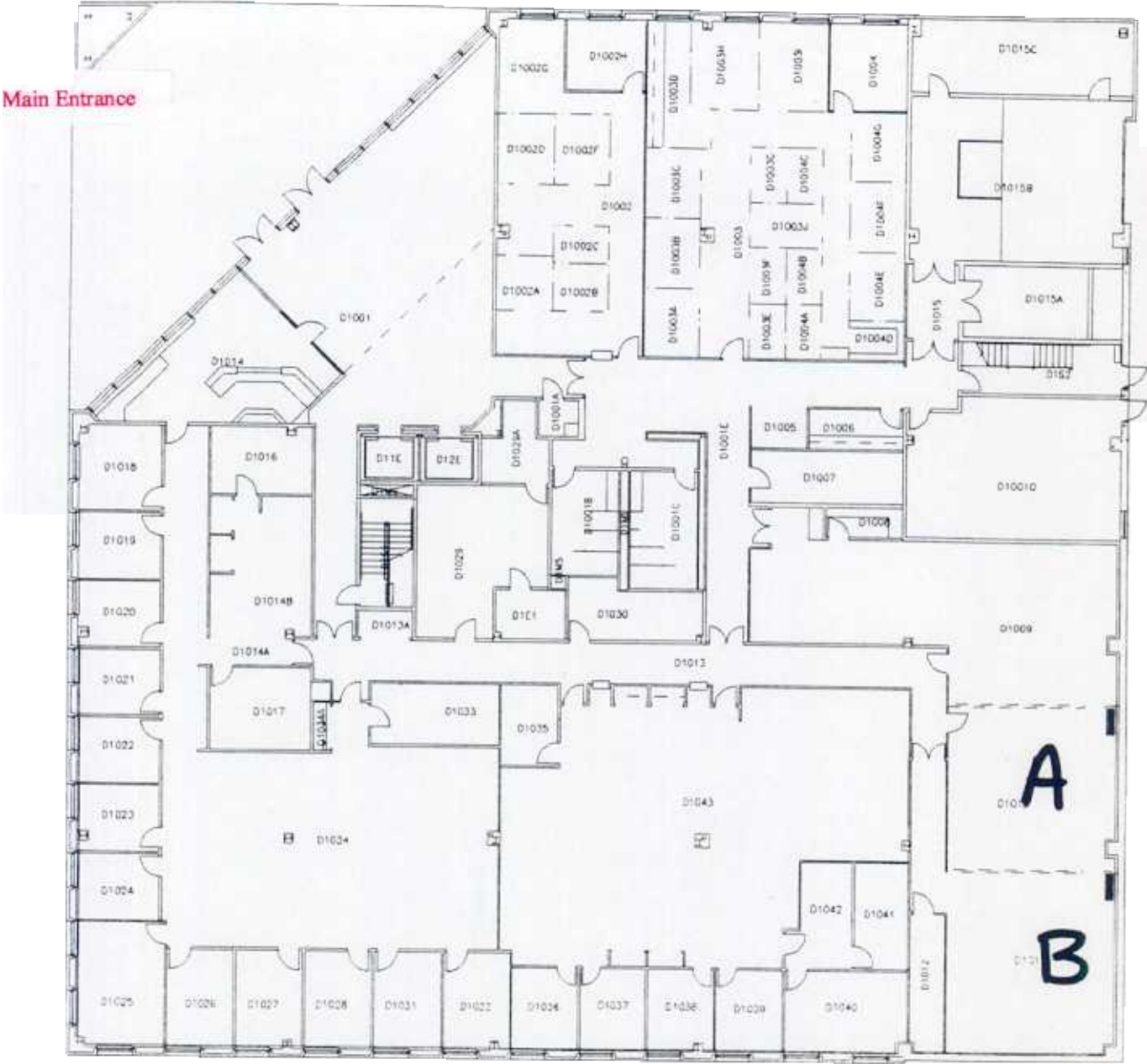
1st FLOOR
